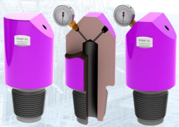
• TYPE SC-V & TYPE SC-W testing Plug and Cup with with one or two NPT outlet for pressure test and pressure dial gauge
